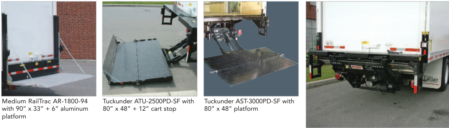
Magnum Tuckunder MTU-GLR-4 with 80" x 60" platform
