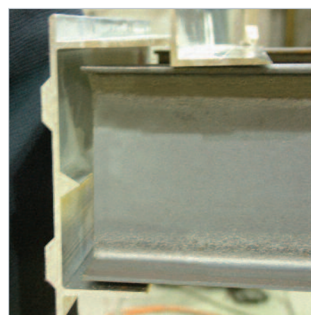
Rub rail with interior V and no exterior bolts
